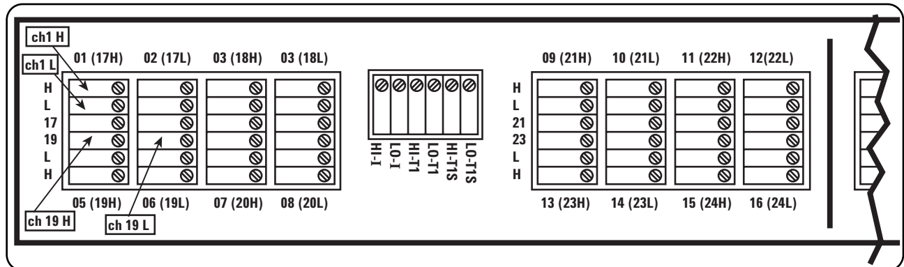
Figure 1: Left side of the E1586A terminal panel, shown with two-wire markings
